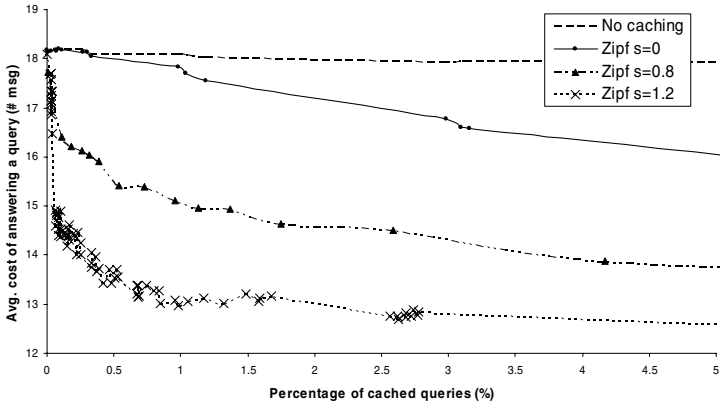
Fig. 4. Average number of messages required to answer a query in the network of 1000 peers depending on the fraction of cached queries
